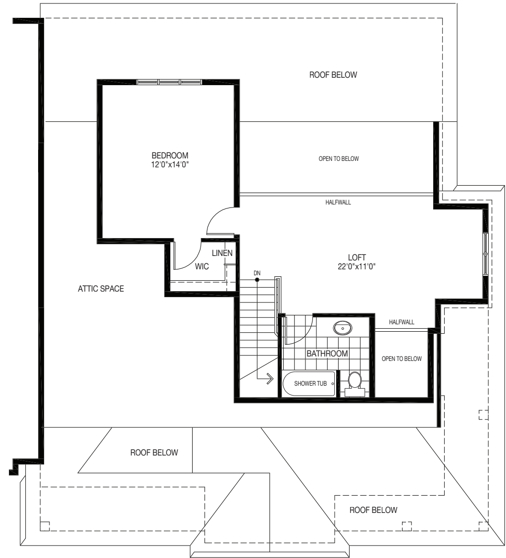
ELEVATION A SECOND FLOOR
