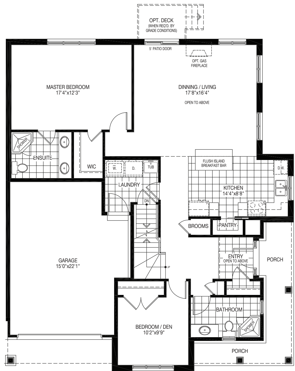
ELEVATION A GROUND FLOOR
